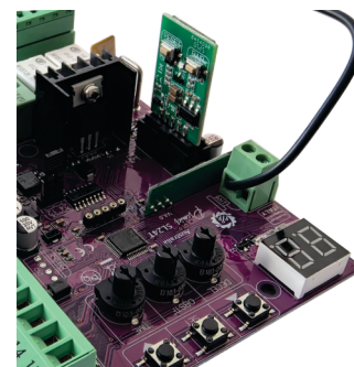
Premier SL24T Sliding Gate Controller (Purple Version)
