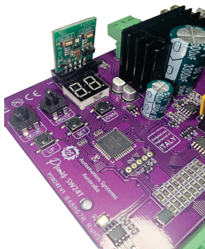
Premier SW24T Swing Gate Controller (Purple Version)
